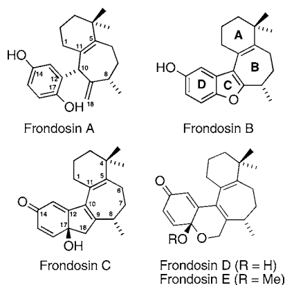
Figure 1. Frondosins A–E.
