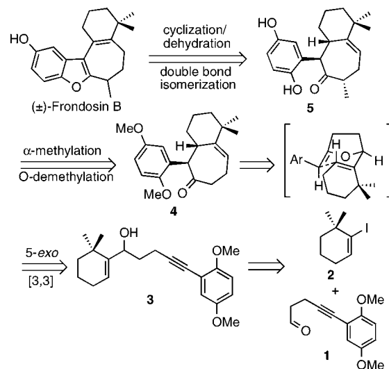
Scheme 1. Retrosynthetic Analysis for the Synthesis of Frondosin B
