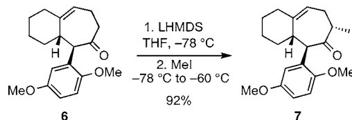
Scheme 2. Synthesis of a Bicyclic Ketone Model System
