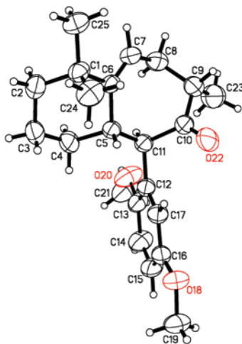
Figure 2. ORTEP drawing of compound 8 derived from a single-crystal X-ray analysis (arbitrary numbering of atoms).
